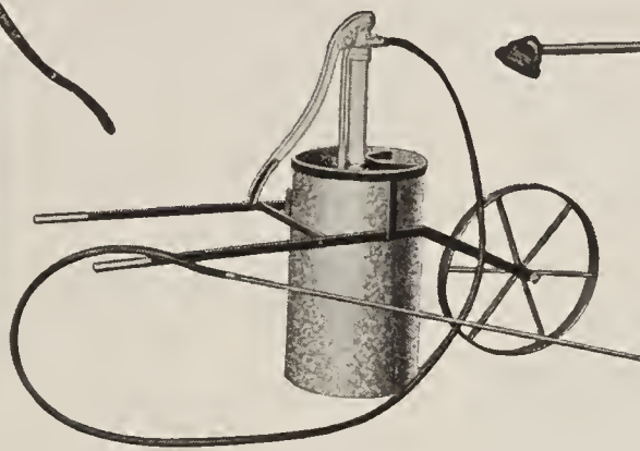
Fig. 832. Outfit A. A small barrel sprayer. 2 gallon per minute at 150 lbs. pressure. Without barrel. Complete with hose and nozzle. $9.50.
